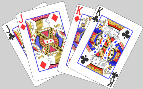
Leduc Hold'em
